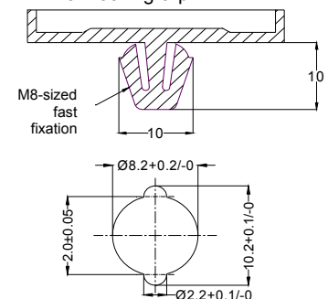
# = 5: Locking clip
