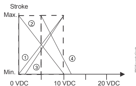
Figure 15: Graphed Examples of Table 3 Command Signals
