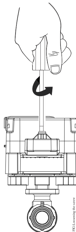
Figure 5: Loosening the Actuator Handle
