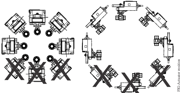
Figure 2: Mounting Positions
