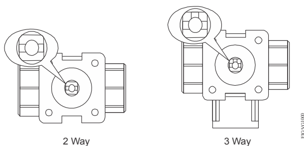
Figure 3: Positioning the Valve Stem
