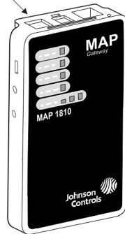
Figure 13: Connecting the Portable MAP Gateway to Your Equipment
