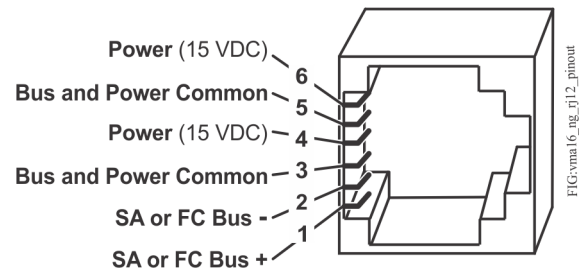
Figure 10: SA/FC Port Pin
