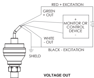
VOLTAGE OUT
